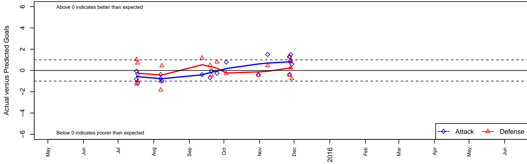
Santa Clara Sporting Black B98 Dots are actual minus expected GF (blue circles) and GA (red triangles). Blue line is smoothed change in attack strength. Red is smoothed change in defense strength.
